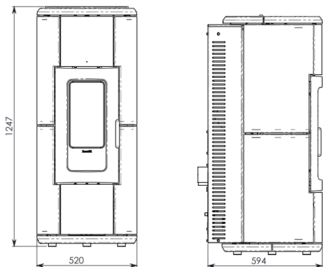
R-Evolution 11 technical diagram
