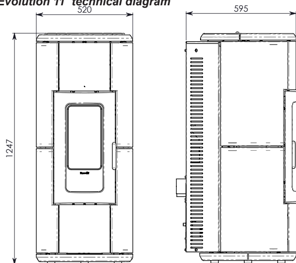
R-Evolution 11 technical diagram
